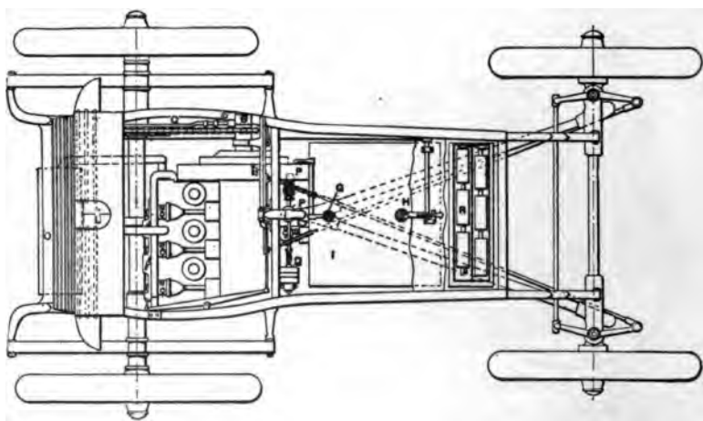
FIG. 269.—Plan View of Duryea Three-cylinder Car. B, bearing for speed gear; C, distance-rod from rear axle for taking up the pull of the chain; D, the magneto-generator; G, pedal for operating the reverse clutch; H, brake pedal; I, gasoline tank; P, central single control lever; R, 6-cell battery. Front axle shorter than rear to prevent skidding and promote ease in turning.
